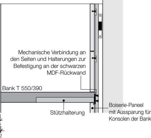
BANK ST 60
