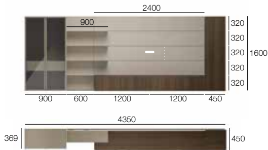
B 4350 x H 1600 x T 369/450
