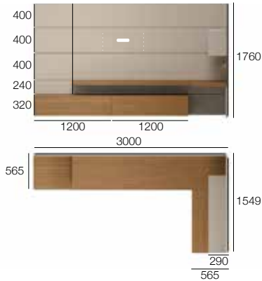
B 3000 x 1549 x H 1760 x T 290/565
